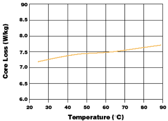
Core Loss vs. Temperature @ 0.1 T/100 kHz
