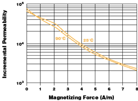
Incremental Permeability vs. dc Bias @ 10 kHz
